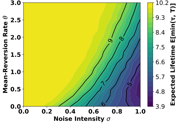
Figure 12: Contour plot of the Expected (truncated) Lifetime \mathbb{E}[\min(\tau, T)] for T = 10 , as a function of noise intensity \sigma and mean-reversion rate \theta with \mu = 0.5 , computed using 2,000 Monte Carlo simulations. Warmer colours indicate longer coherence lifetimes, highlighting the tradeoff between environmental noise and stabilizing system dynamics.
