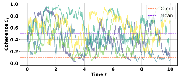
Figure 5: Sample paths of the qubit coherence process C_t after transforming from Y_t , ensuring bounded dynamics. The dashed line in red is the critical threshold C_{crit} , and the one in violet is the baseline coherence. The trajectories are within the required interval (0,1) .
