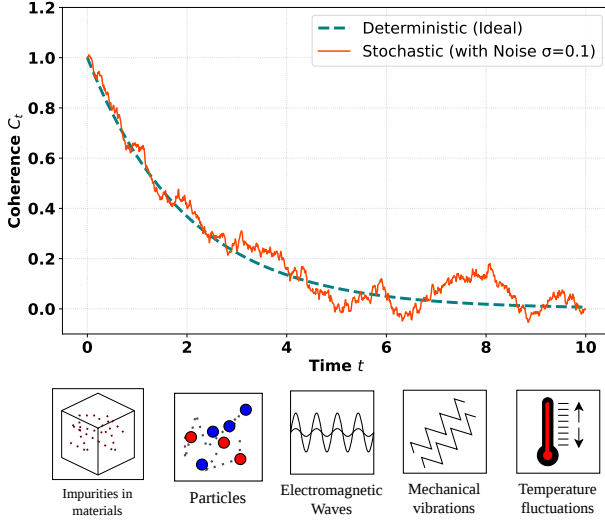
Figure 2: Plot: Exponential Coherence Decay - Deterministic (teal) vs Noisy Environment (orange). Elements: Types of environmental noise like (in order from left to right) impurities in materials, particles, electromagnetic waves, mechanical vibrations, and temperature fluctuations.
