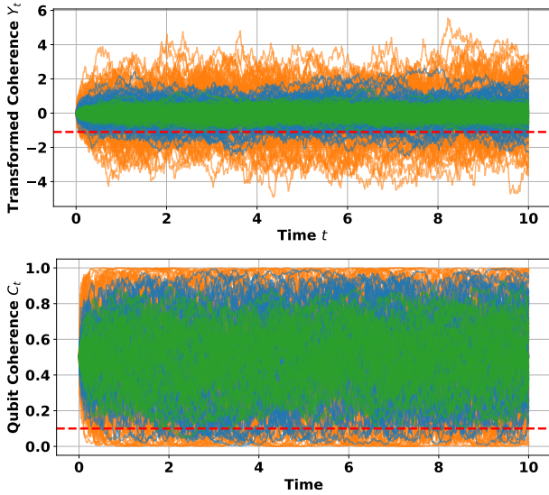
Figure 8: Sample trajectories of the Transformed Coherence Y_t (top) and Qubit Coherence C_t (bottom) for different Noise Intensity \sigma values of 0.5 (green), 1.0 (blue), and 2.0 (orange), each plotting 100 realizations. The long-term mean coherence and mean-reversion rate were fixed at \mu = 0.5 and \theta = 1.0 . The red dashed line represents the C_{crit} threshold. Increasing \sigma produces larger fluctuations in the process, making threshold crossings and decoherence events more likely.
