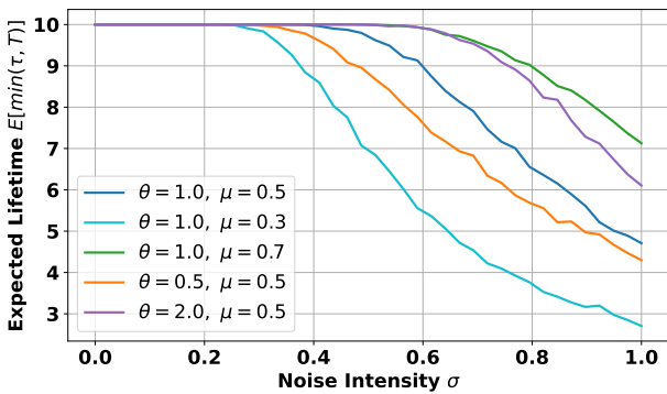
Figure 11: Expected (truncated) Lifetime \mathbb{E}[\min(\tau, T)] as a function of noise intensity \sigma for several parameter configurations: \theta = 1.0, \mu = 0.5 (blue), \theta = 1.0, \mu = 0.3 (cyan), \theta = 1.0, \mu = 0.7 (green), \theta = 0.5, \mu = 0.5 (orange), and \theta = 2.0, \mu = 0.5 (purple), computed using 2,000 Monte Carlo simulations for each curve. The curves illustrate how increasing environmental noise reduces the average duration for which the qubit remains above the coherence threshold. Variations in \mu and \theta demonstrate the stabilizing effects of higher mean coherence and stronger mean-reversion.
