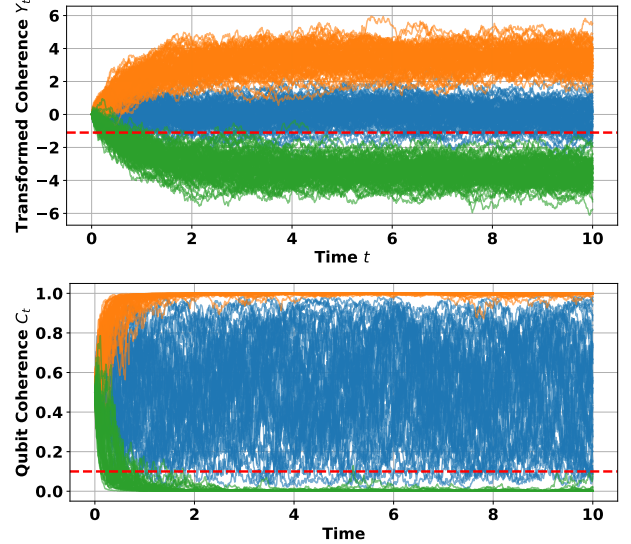
Figure 6: Sample trajectories of the Transformed Coherence Y_t (top) and Qubit Coherence C_t (bottom) for different Long-Term Mean Coherence \mu values of 0.001 (green), 0.5 (blue), and 0.999 (orange), each plotting 100 realizations. The mean-reversion rate and noise intensity were fixed at \theta = 1.0 and \sigma = 1.0 . The red dashed line represents the C_{\text{crit}} threshold. Increasing \mu shifts the equilibrium level of the process upward, resulting in trajectories that fluctuate around higher coherence levels.
