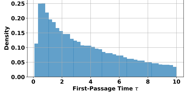
Figure 9: Histogram of simulated first-passage times \tau , defined as the first time the coherence process falls below the threshold C_{crit} . The parameter values for the simulations were set at \mu = 0.5 , \theta = 1.0 , and \sigma = 1.0 . The distribution illustrates the variability in decoherence times across 100,000 Monte Carlo realizations due to stochastic environmental fluctuations.
