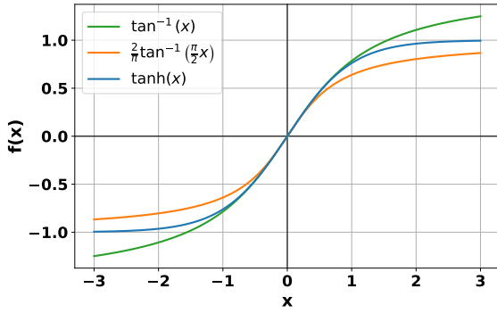
Figure 4: Comparison of candidate transformations mapping \mathbb{R} to bounded intervals.
