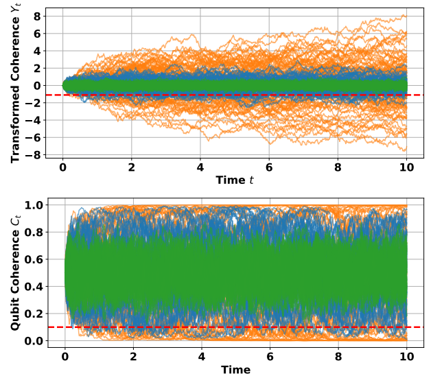
Figure 7: Sample trajectories of the Transformed Coherence Y_t (top) and Qubit Coherence C_t (bottom) for different Mean-Reversion Rates \theta of 0.05 (orange), 1.0 (blue), and 8.0 (green), each plotting 100 realizations. The long-term mean coherence and noise intensity were fixed at \mu = 0.5 and \sigma = 1.0 . The red dashed line represents the C_{\text{crit}} threshold. Increasing \theta causes the process to return more rapidly toward its equilibrium level, resulting in smaller deviations from the long-term mean coherence.
