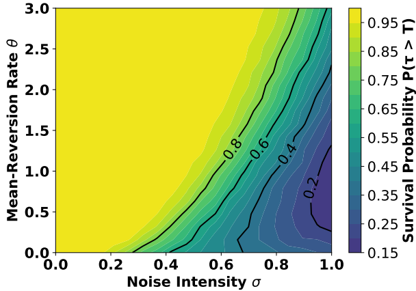
Figure 13: Contour plot of the Survival Probability P(\tau > T) , representing the probability that the qubit remains coherent throughout the computation interval T = 10 , as a function of noise intensity \sigma and mean-reversion rate \theta with \mu = 0.5 , computed using 2,000 Monte Carlo simulations. The plot shows how increasing noise reduces reliability, while larger mean-reversion rates improve coherence stability.
